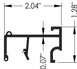
38 SIDELITE ADAPTER Endura
