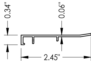
39 SIDELITE ADAPTER Endura
