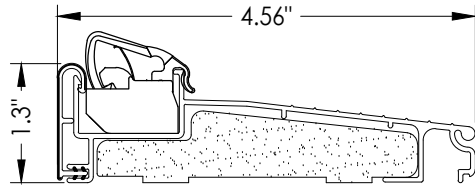
34 INSWING THRESHOLD Endura (Articulating) ALUM/COMP/VINYL
